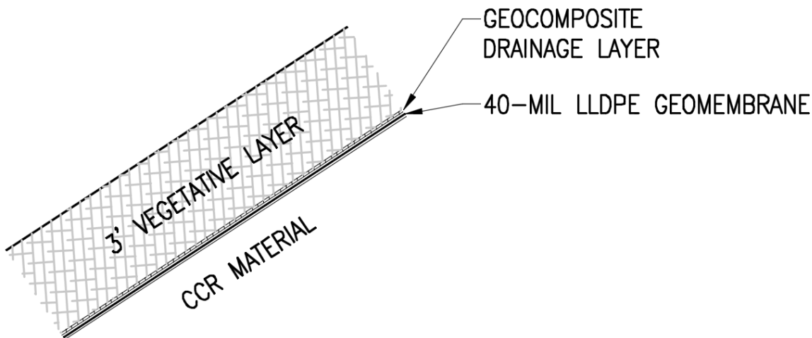
Figure 3-1 Composite Final Cover
